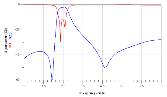
RFBPF2012080AFT
