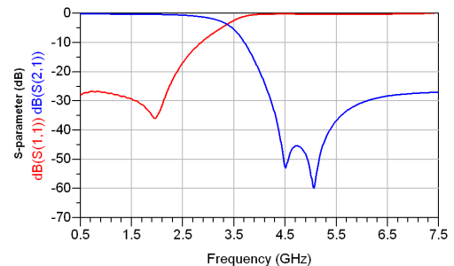
RFLPF160806A0T
