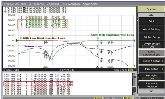
RFDIP2012100L0T
