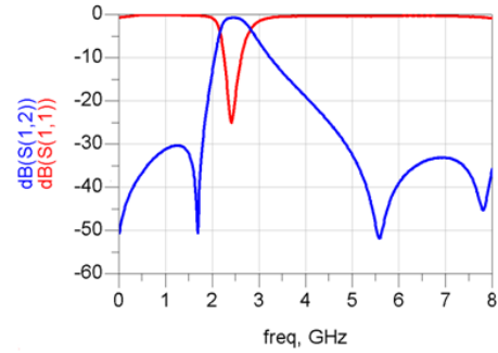
RFBPF2012050ACT
