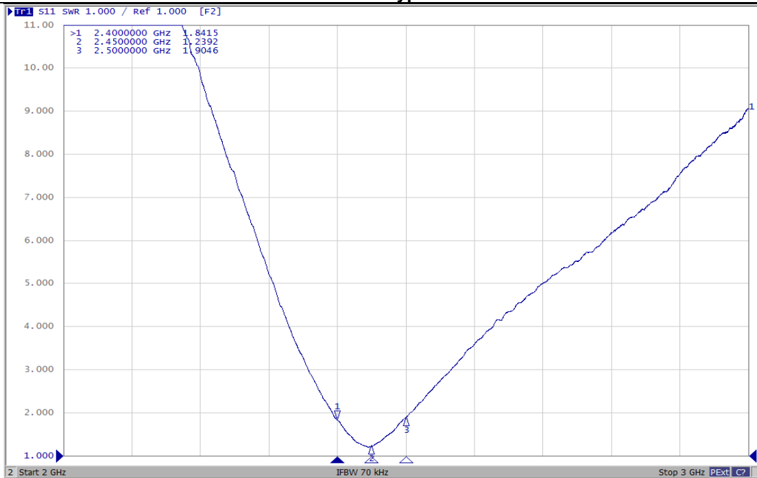
Antenna VSWR on Type-1 Test Board
