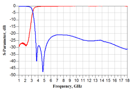
RFLPF1608060AAT
