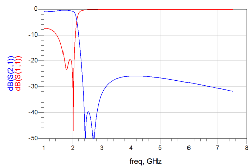
RFLPF1005040A1T
