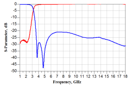
RFLPF160806A0T
