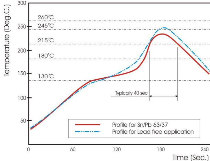
Fig 3. Infrared soldering profile for Chip Resistors WW12
