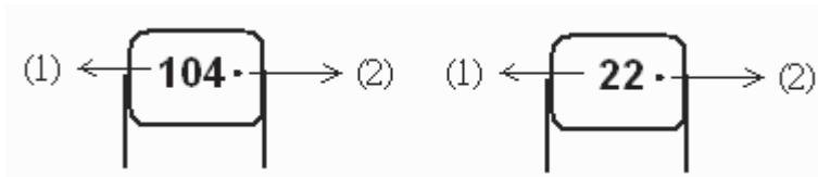
3-figure code Marking
