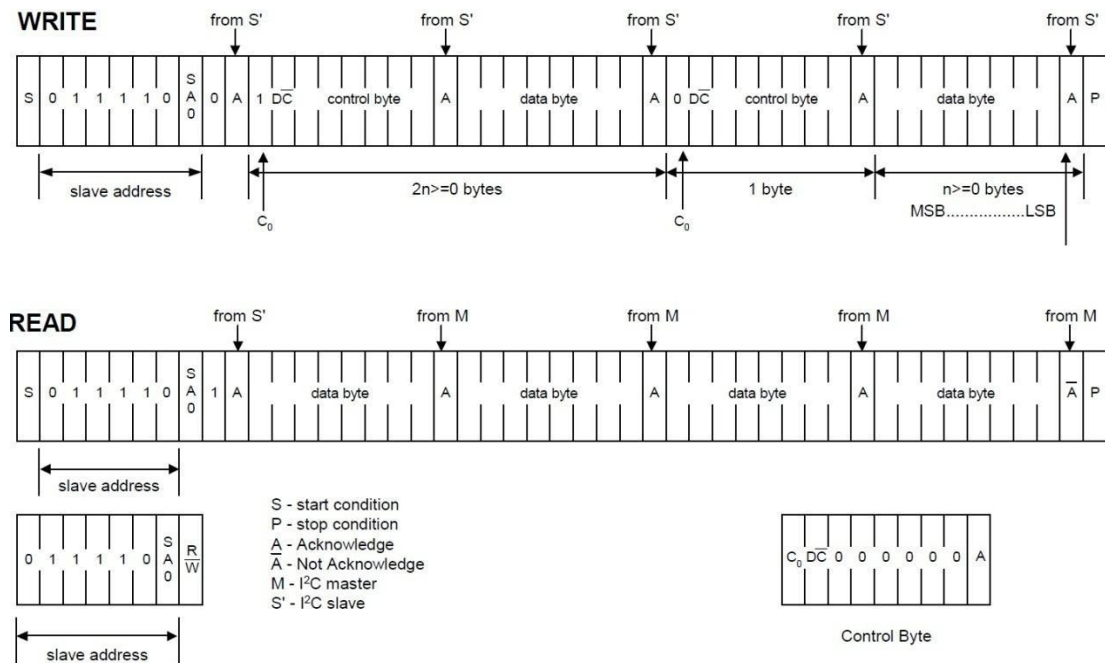
Figure 6: I2C Protocol
