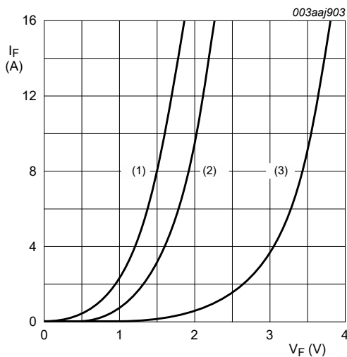
V_o = 1.581\text{ V}; R_s = 0.043\ \Omega (1) T_j = 125\text{ °C}; typical values (2) T_j = 125\text{ °C}; maximum values (3) T_j = 25\text{ °C}; maximum values
