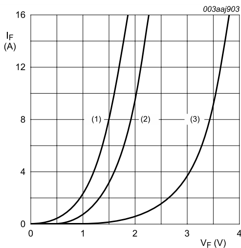
(1) T_j = 125\text{ °C} ; typical values (2) T_j = 125\text{ °C} ; maximum values (3) T_j = 25\text{ °C} ; maximum values V_o = 1.581\text{ V}; R_s = 0.043\ \Omega
