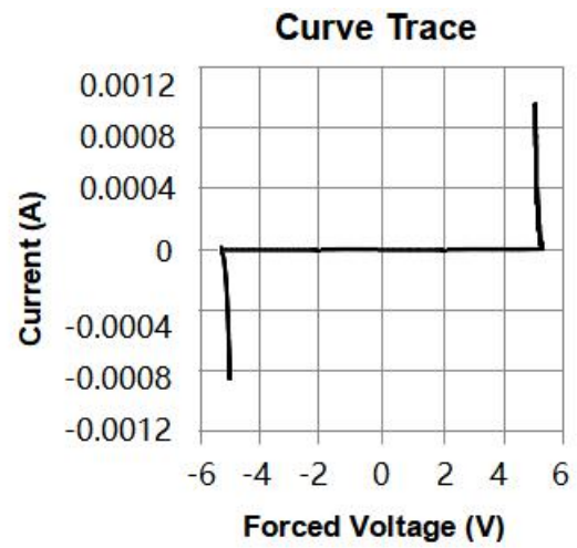
Fig.4 IV Curve
