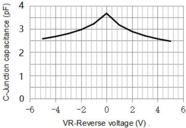
Fig.3 Capacitance vs. Reverses Voltage
