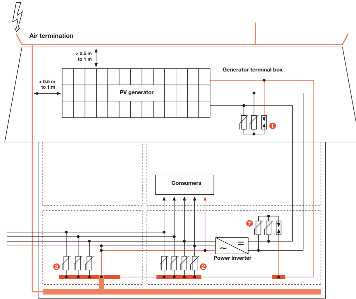
(example drawing: no liability taken)
