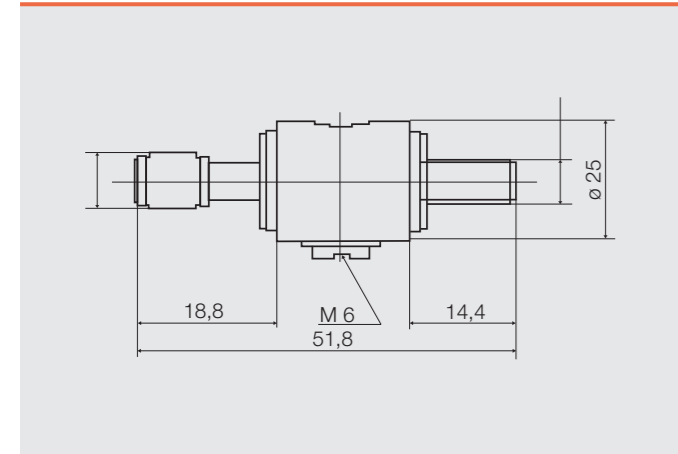
F Connector / M-F
