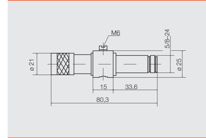
N Connector / M-F
