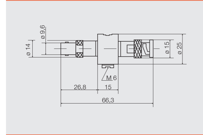
BNC Connector / M-F
