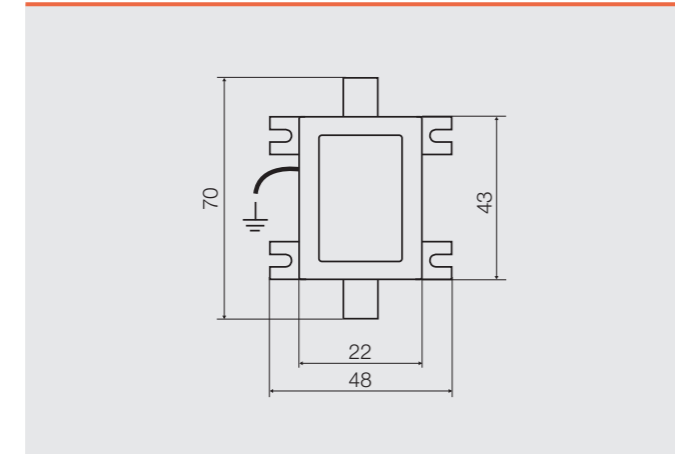
UHF Connector / M-F
