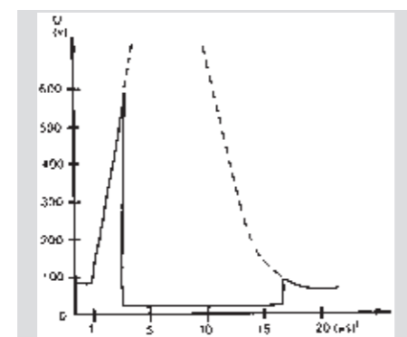
DK 4 U gas discharge tube 5 kA, 90 V
