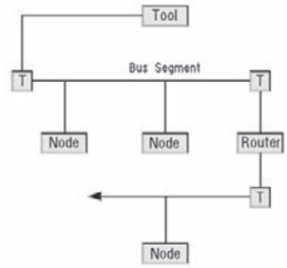
TP / XF Multidrop Bus Topology (J3)
