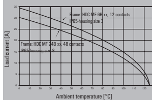
HDC-MHE 6-modules in the IP65-housing, Conductor H07V-K4.0:
