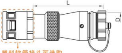
塑料软管接头可选购 Optional plastic hose adapter
