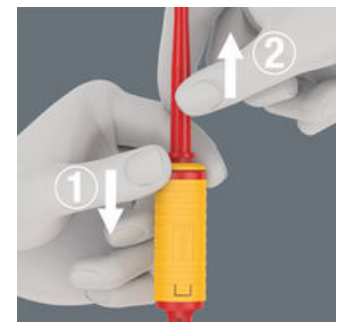
By pulling and holding down the clamping sleeve the interchangeable screwdriver blade, or the switch cabinet key, is unlocked and can easily be taken out of the handle.
