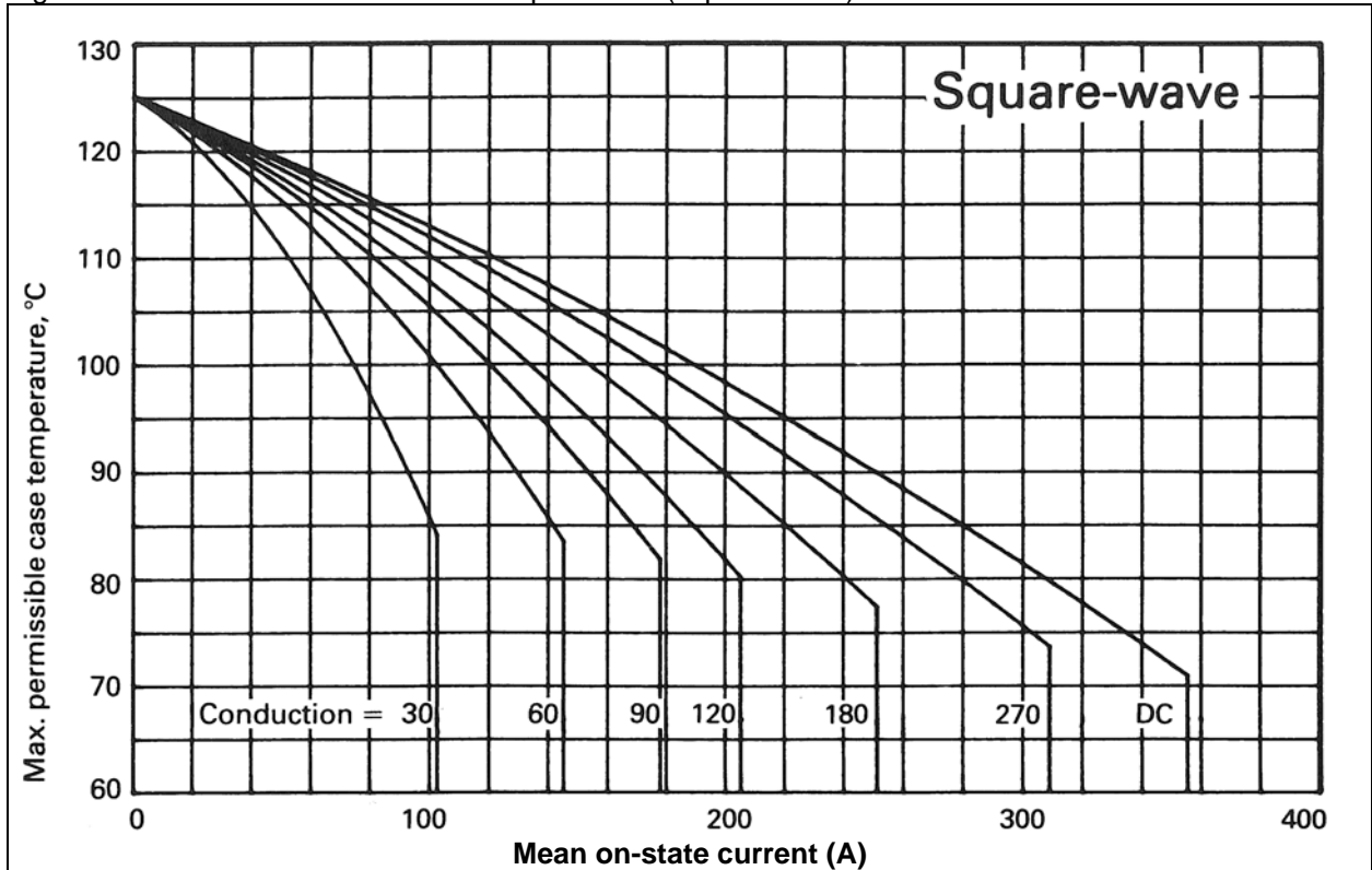
Figure 7 – On-state current vs. case temperature - (Square wave)
