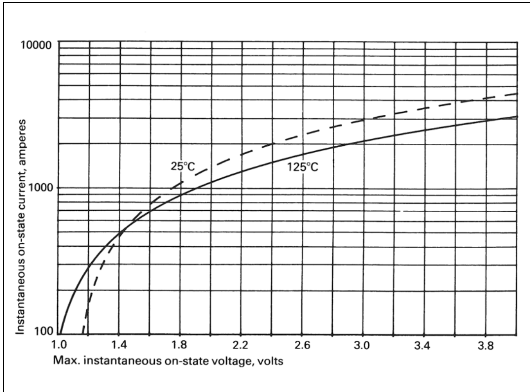
Figure 1 - On-state characteristics of Limit device
