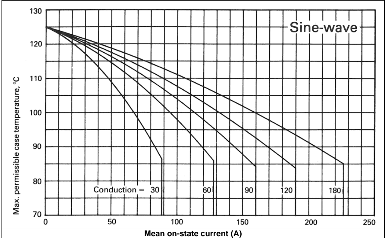
Figure 5 – On-state current vs. case temperature - (Sine wave)
