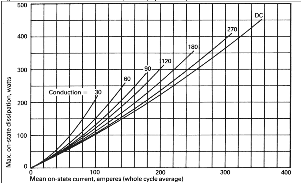
Figure 8 – On-state current vs. Power dissipation - (Square wave)
