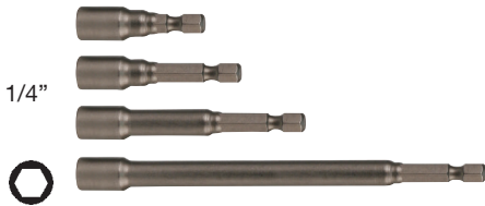
704 Nut Setters Standard. 1/4" Hex Inch Permanent industrial magnet.
