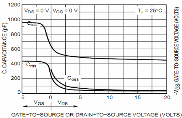
Capacitance Variation
