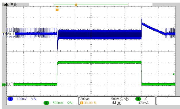
Load Transient Response VIN=5V, VO=1.8V, EN=3.6V, IO=1mA-1A
