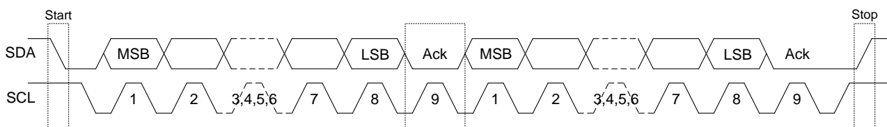
Fig5 I2C data transactions
