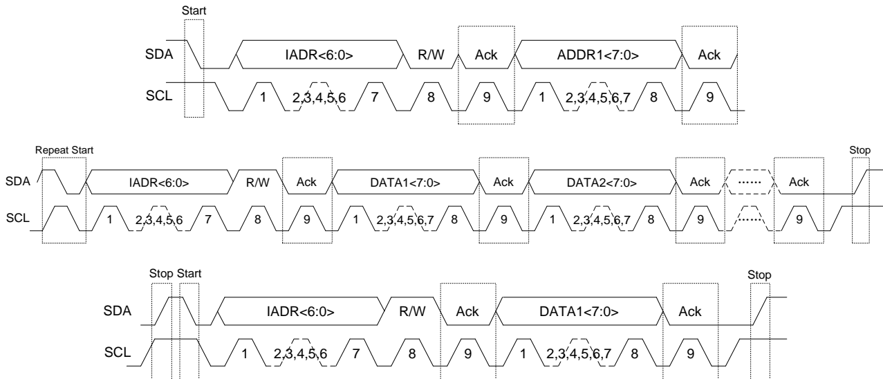
Fig7 I 2 C Read Cycle
