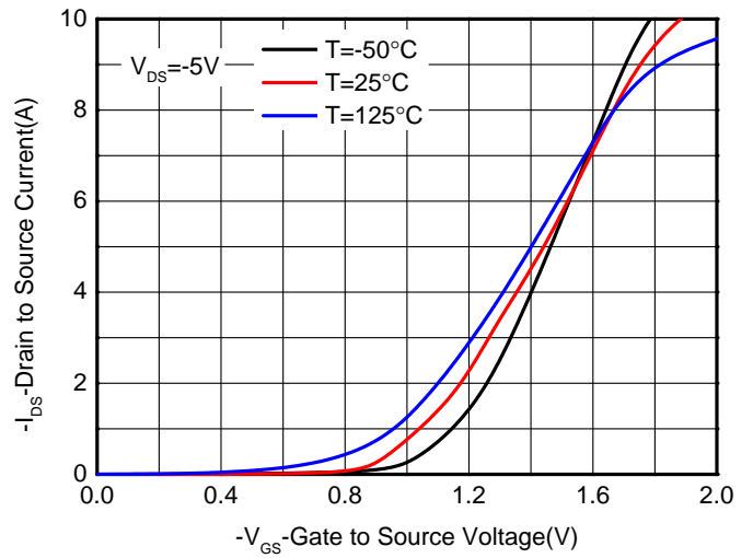
Transfer characteristics
