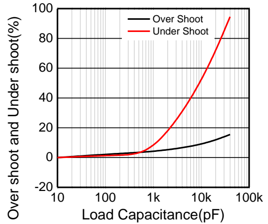
Over-Shoot % vs. C_{\text{load}}
