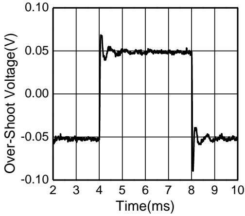
Over-Shoot Voltage
