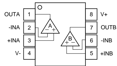
SOP-8L/MSOP-8L
