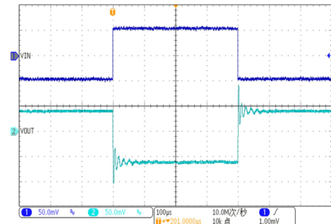
Over Shoot Voltage, C_{load}=47\text{nF} , R_{load}=40\text{k}\Omega , Gain=-1
