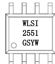
SOP-8L
