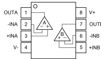
MSOP-8L
