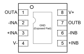
DFN2x2-8
