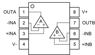
SOP-8L/MSOP-8L /TSSOP-8L/SOT23-8L Pin configuration (Top view)
