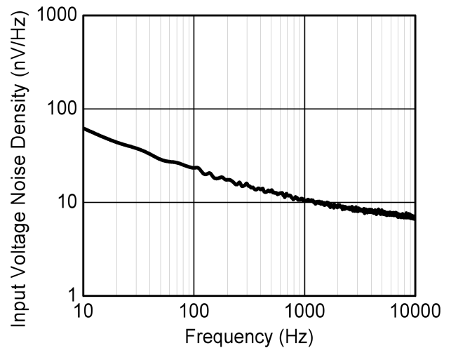
Noise Density
