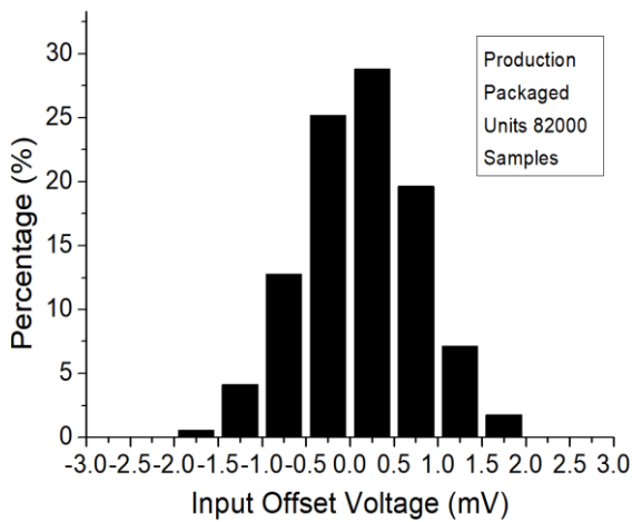
Input Offset Voltage Distribution
