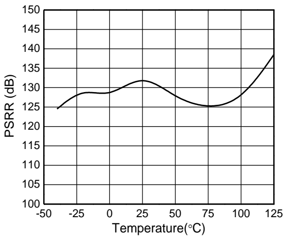
PSRR vs. Temperature
