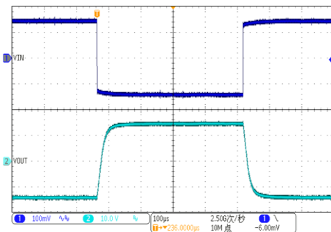
Negative/Positive Over-Voltage Recovery
