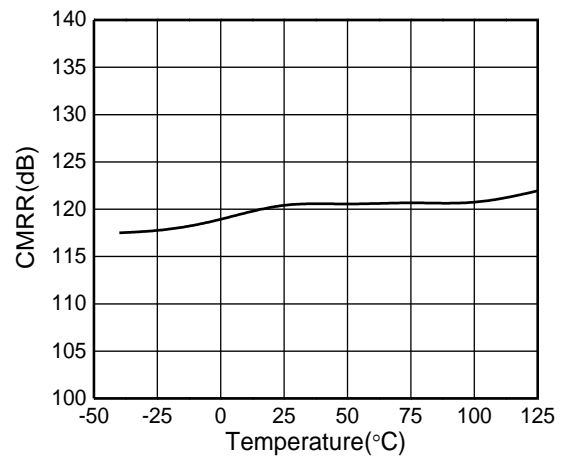
CMRR vs. Temperature
