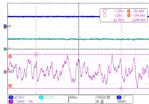
0.1Hz to 10Hz Integrated Input Noise, Gain = 50000
