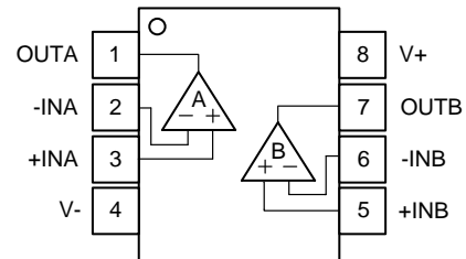
SOP-8L/MSOP-8L
