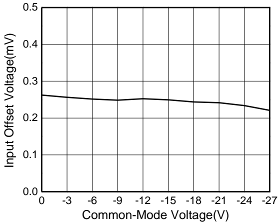
Input Offset Voltage vs. Common-Mode Voltage
