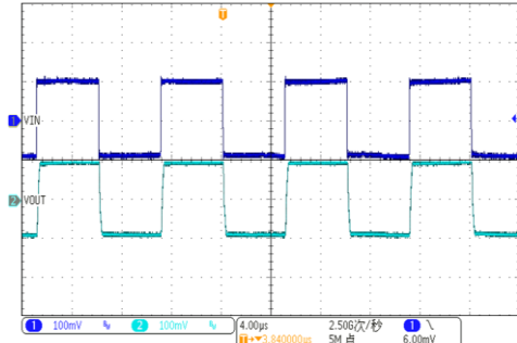
Small-Signal Step Response, 100mV Step
