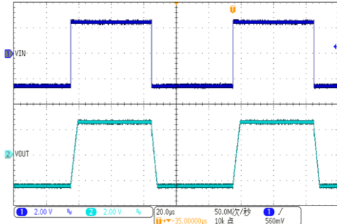
Large-Signal Step Response, 2V Step
