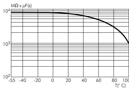
Insulation resistance change versus temperature (general guide)
