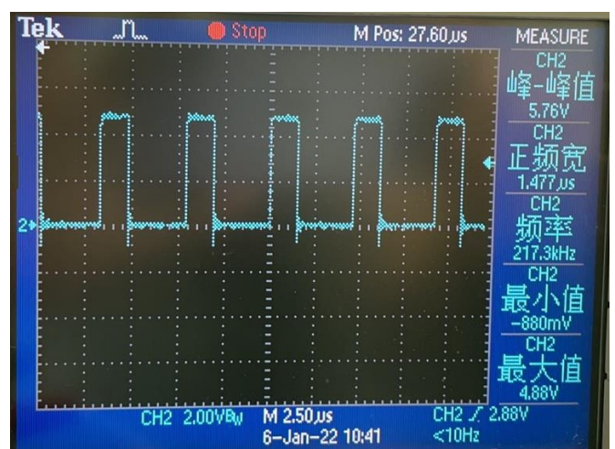
MOS switch waveform
