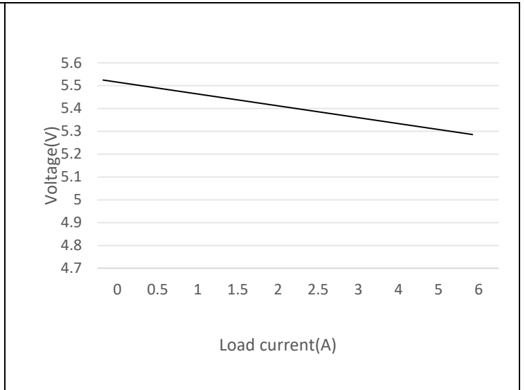
Output voltage (input 48V)
