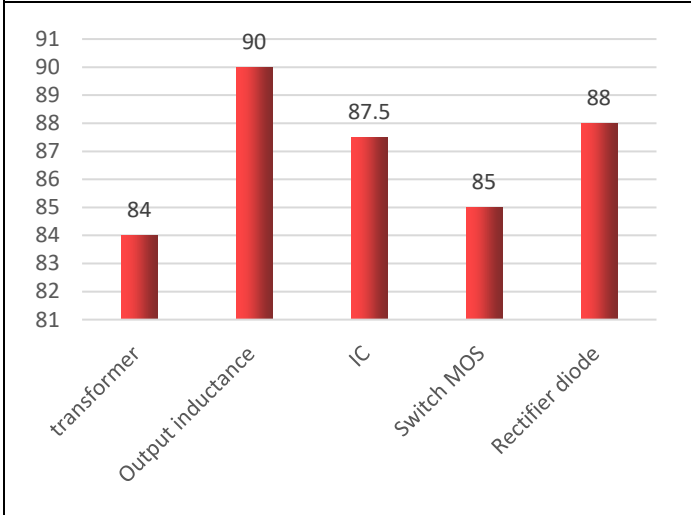
Maximum temperature of components Conditions (ambient temperature: 27 °C; output power: 5.5V / 5A; frequency: 3H)
