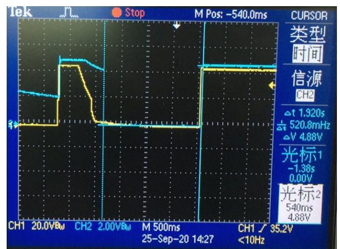
Output response & load (5.5V / 5A)
