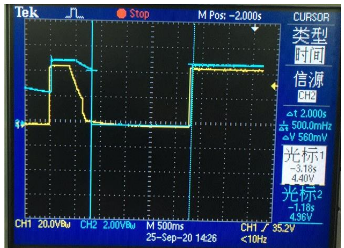
Output response & load (5.5V / 3A)
