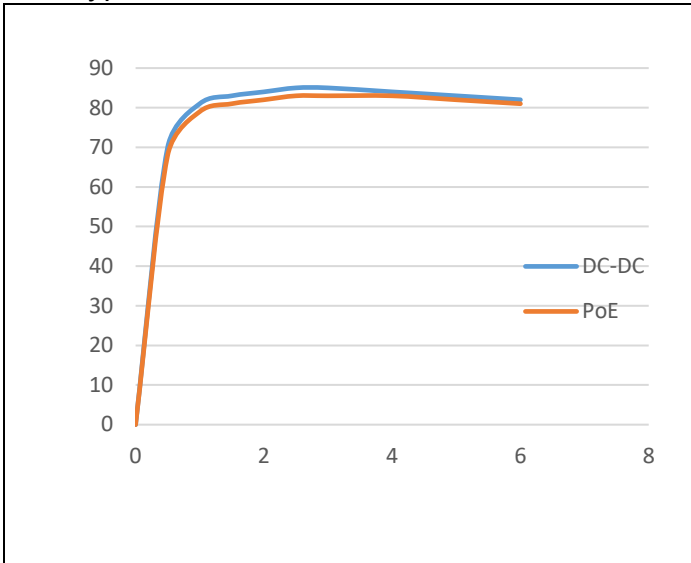
Efficiency (Vout = 5V)
