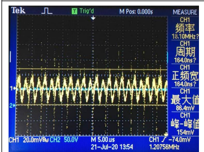
Noise (VIN = 48V, IO = 1.25A, 5 ~ 20MHz bandwidth)
