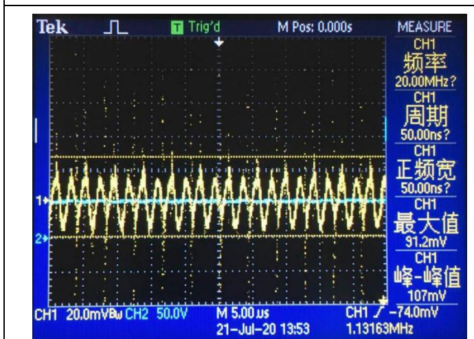
Noise (VIN = 57V, IO = 1.25A, 5 ~ 20MHz bandwidth)
