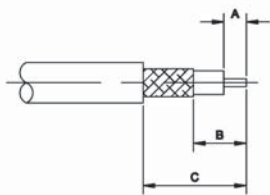
1. STRIP CABLE TO DIMENSIONS AS SHOWN.
