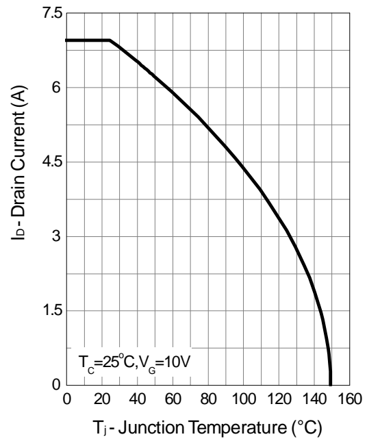
Drain Current
