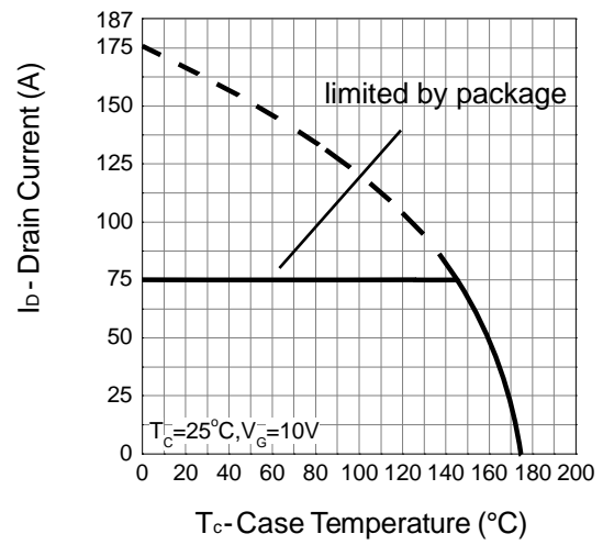
Drain Current
