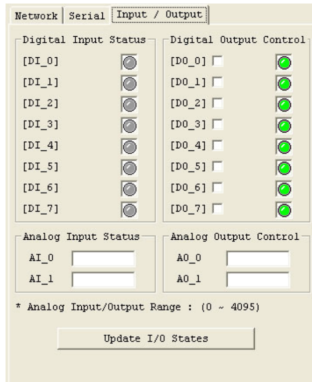
Figure 11. Input / Output Tab of the Configuration Tool
