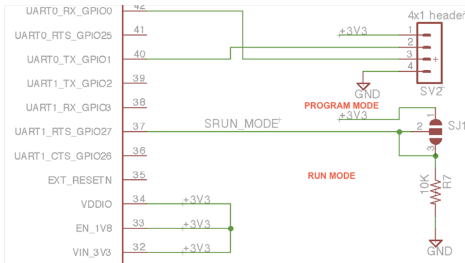
Figure 2 Schematic for mode setting and UART
