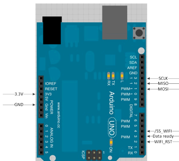
Figure 1 Pins to connect Arduino UNO
