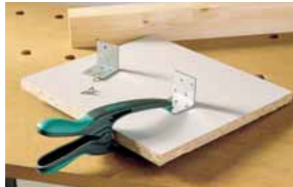
large depth offered by the long clamp arms allows fixing in areas far away from the edge of the workpiece
