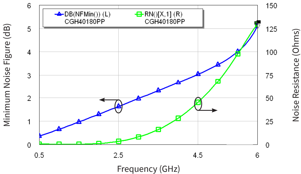
Simulated Minimum Noise Figure and Noise Resistance vs Frequency of the CGH40180PP
