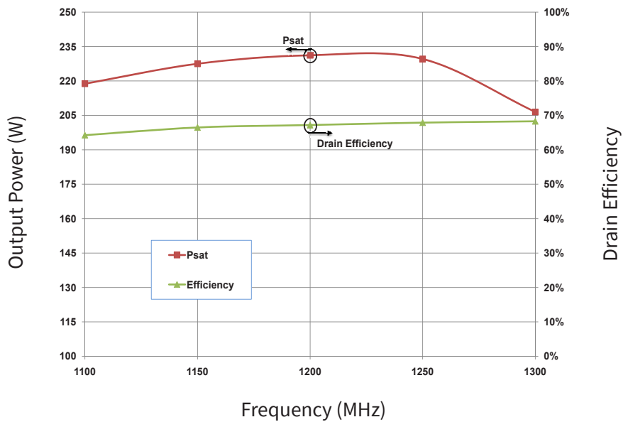
Output Power and Drain Efficiency vs Frequency measured in Broadband Amplifier Circuit CGH40180PP-AMP V_{DD} = 28\text{ V}, I_{DQ} = 2.0\text{ A}
