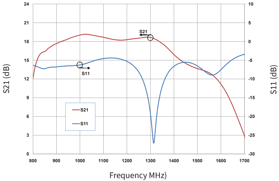
Gain and Return Loss vs Frequency measured in Broadband Amplifier Circuit CGH40180PP-AMP V_{DD} = 28\text{ V}, I_{DQ} = 2.0\text{ A}
