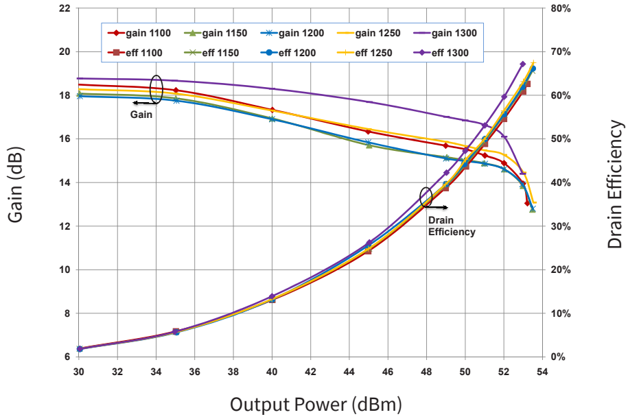
Gain and Drain Efficiency vs Output Power measured in Broadband Amplifier Circuit CGH40180PP-AMP V_{DD} = 28\text{ V}, I_{DQ} = 2.0\text{ A}
