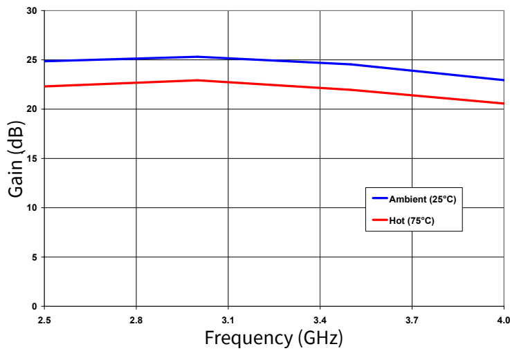
Gain at P OUT of 40 dBm at 25°C & 75°C vs Frequency
