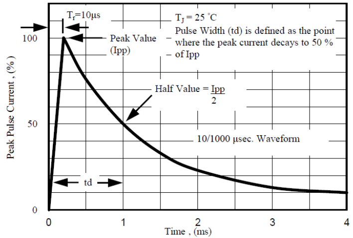
Fig. 2 - Pulse Waveform
