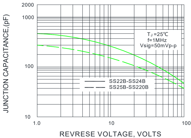
FIG.5-TYPICAL JUNCTION CAPACITANCE
