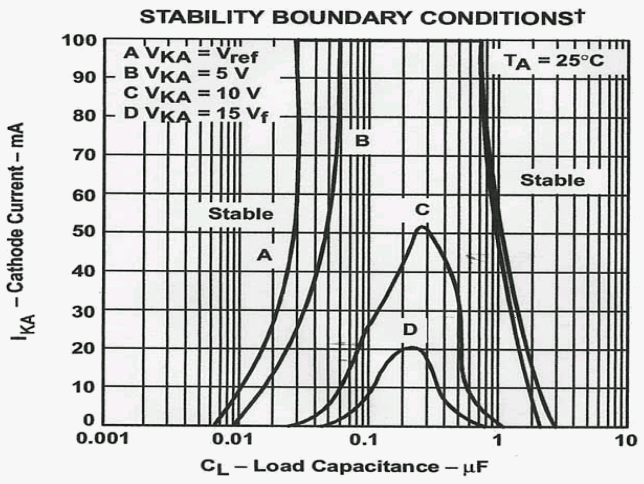
Figure 13. Shunt Regulator
