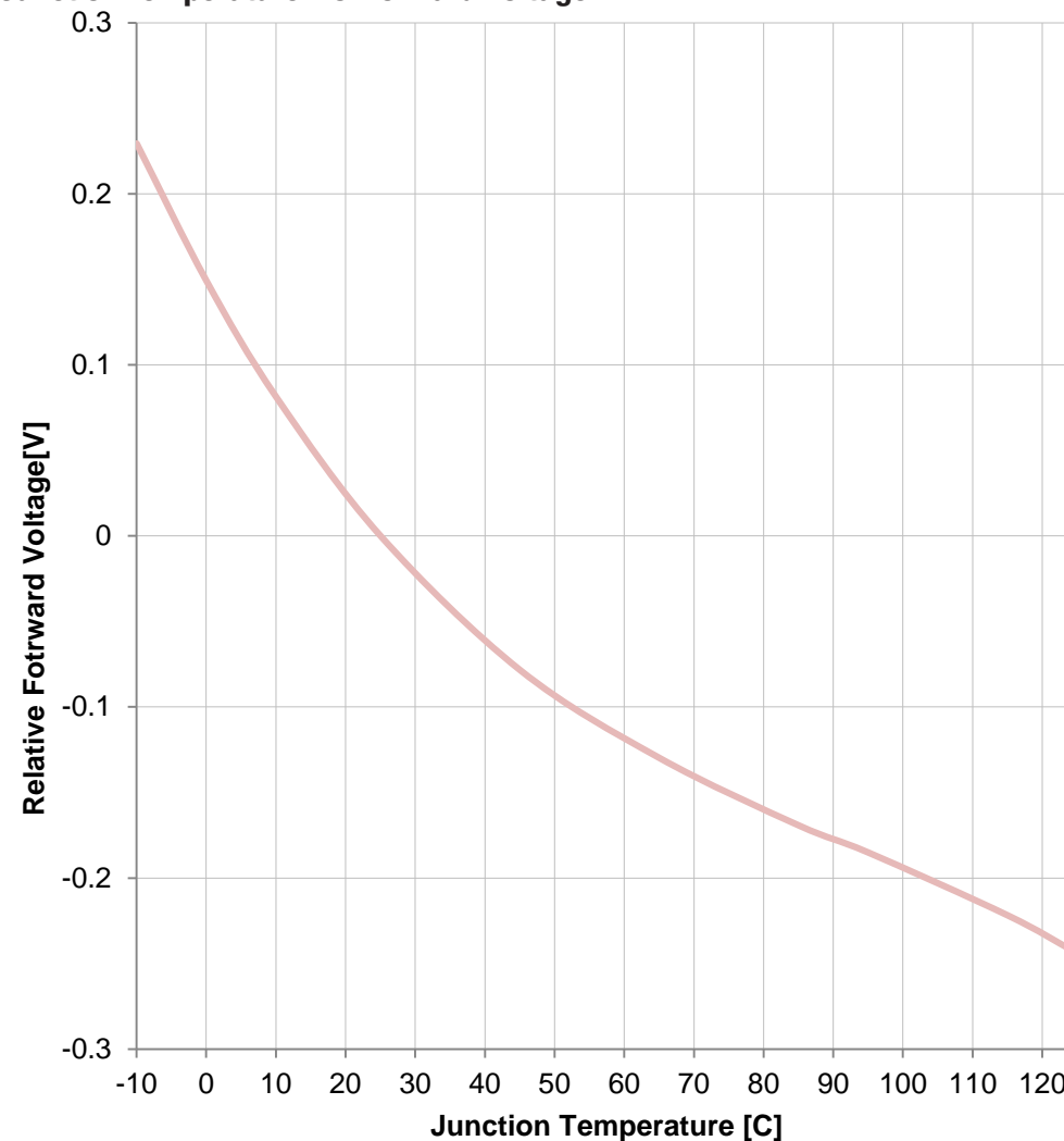
Junction Temperature vs. Forward Voltage:
