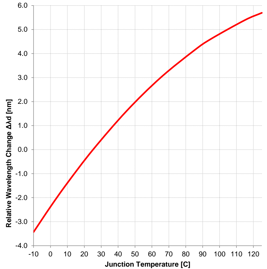
Junction Temperature vs. Dominant Wavelength:
