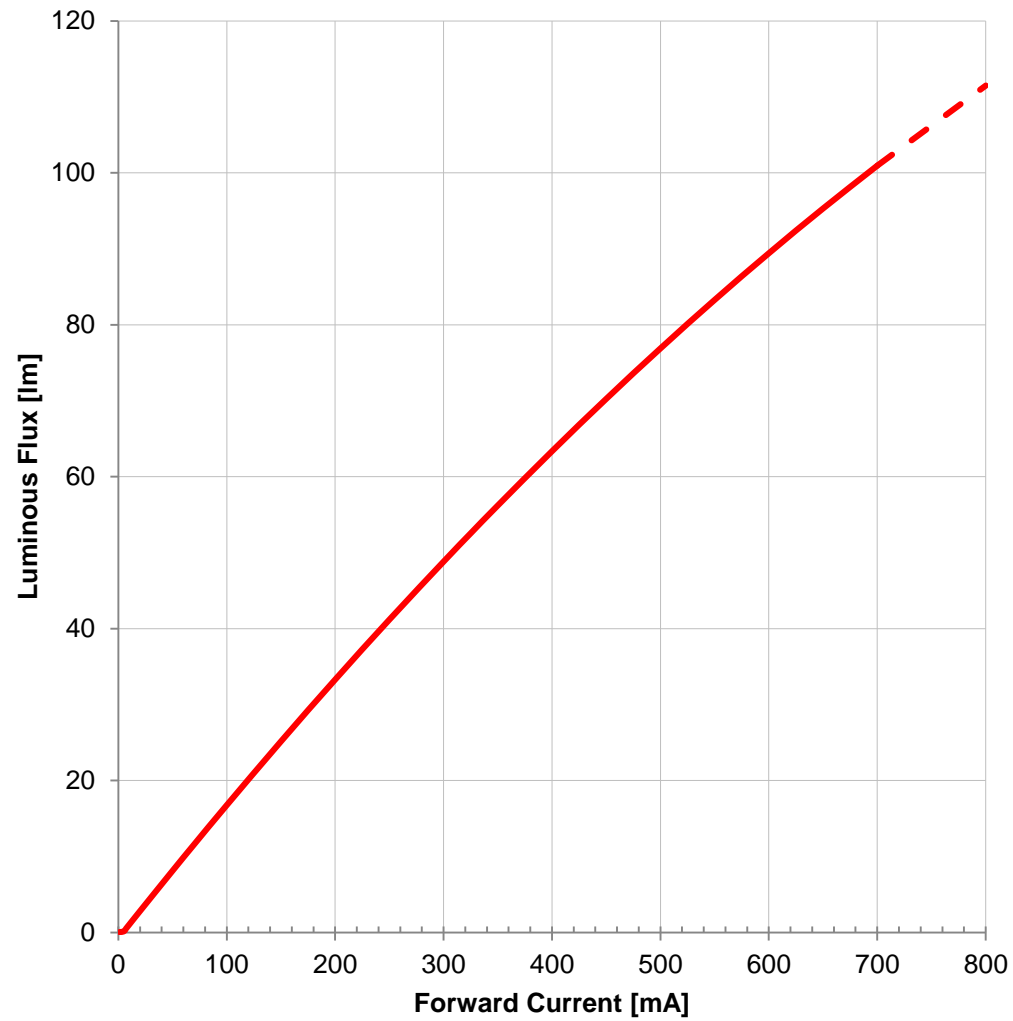
Luminous Flux vs. Forward Current:
