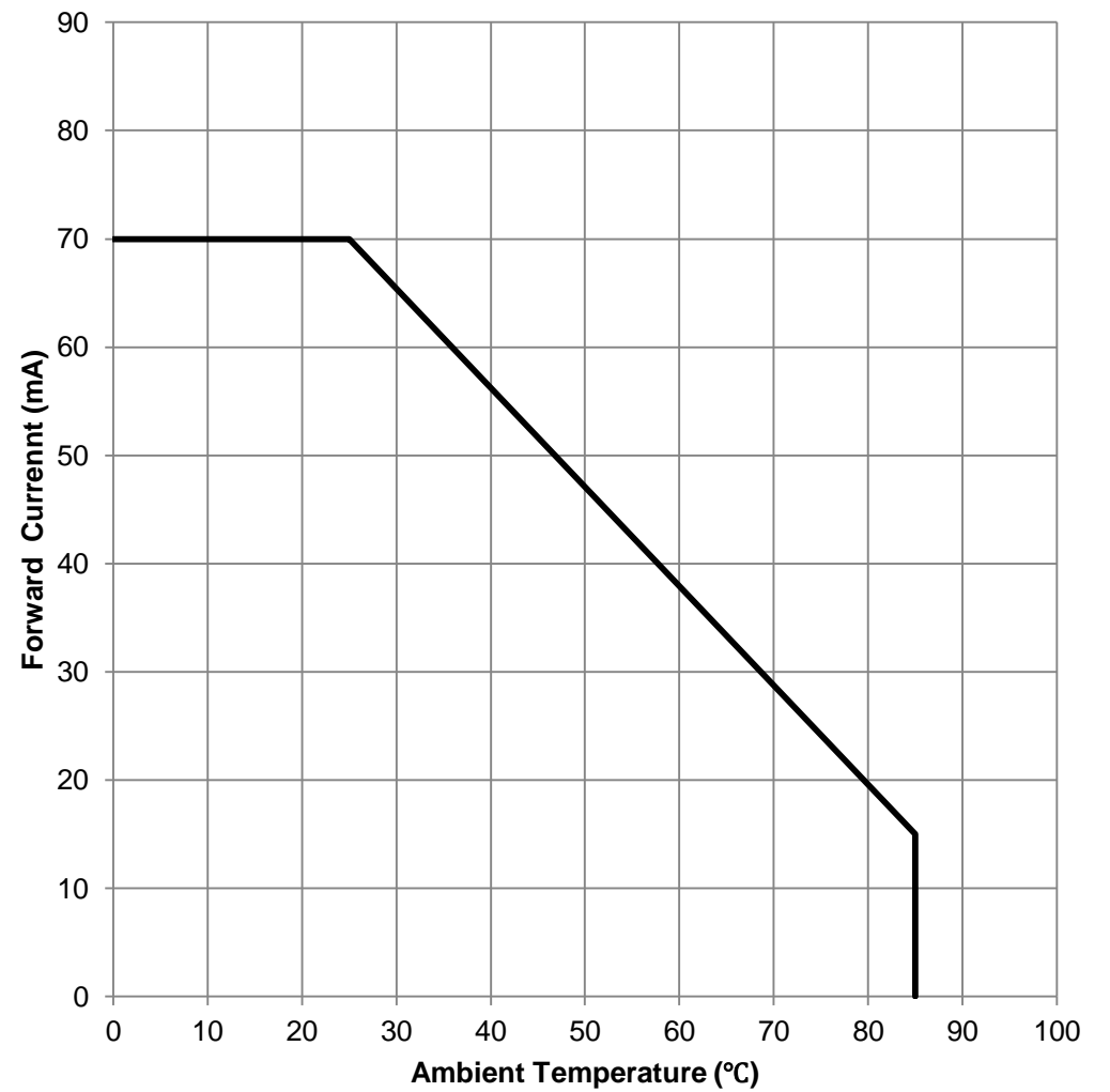
Derating Curve:
