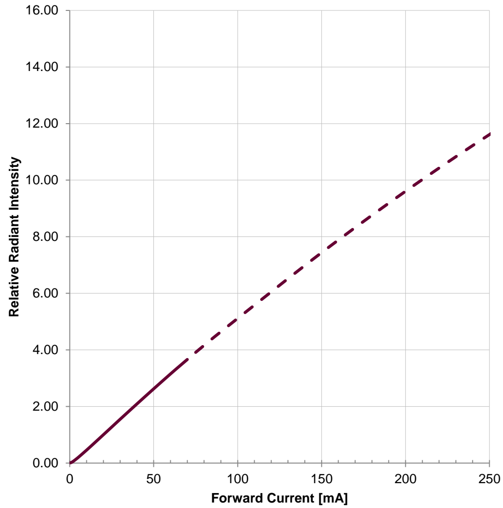
Relative Radiant Intensity vs. Forward Current:
