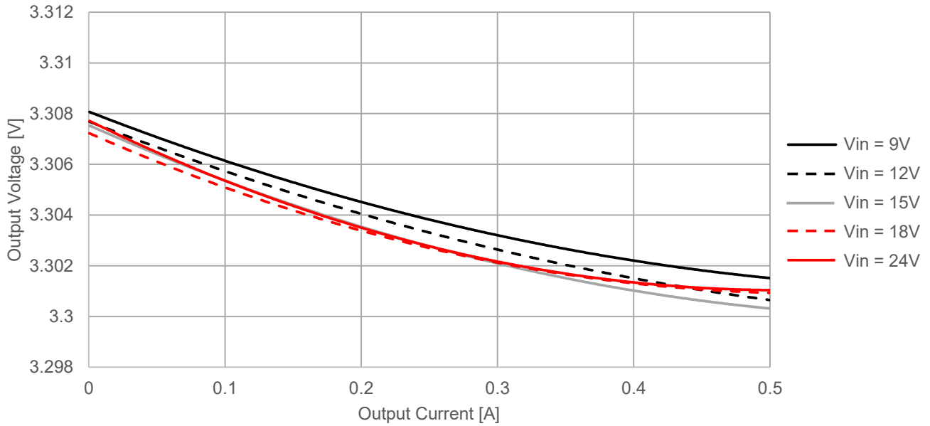
173950336 Load Regulation V_{OUT} = 3.3V , T_A = 25^\circ C
