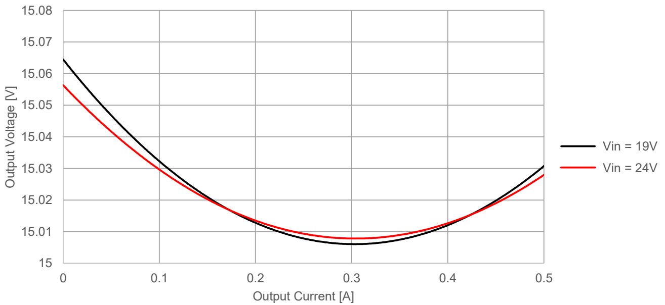
173951536 Load Regulation V_{OUT} = 15V , T_A = 25^\circ C
