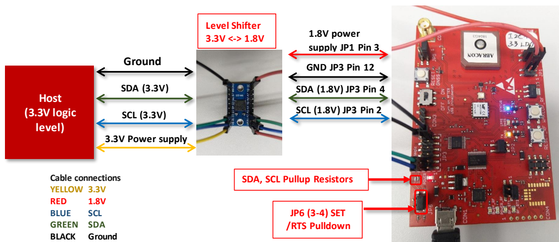
Figure 16: Elara-I- GNSS shifter evaluation board connection to 3.3V Host
