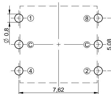
RECOMMENDED LAYOUT
