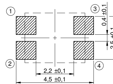
P.C.B MOUNTING PLAN
